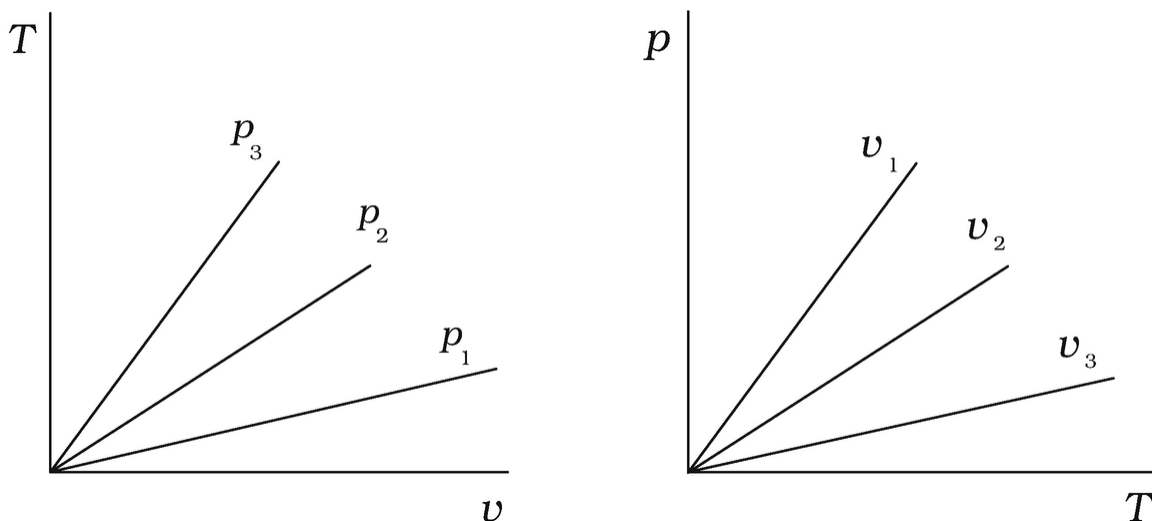
Fig. 2.3 Contour maps for the surface shown in the previous figure
