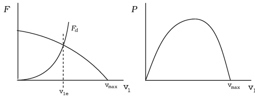
Fig. 6.20 The thrust and propulsive power by a jet engine as a function of flight speed, v_1 . The equilibrium flight speed, v_{1e} , corresponds to the value for which the thrust and drag, F_d , forces are equal
