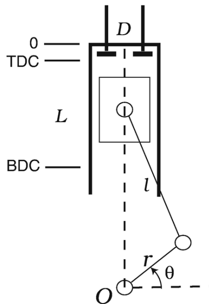
Fig. 6.10 Schematic of a four stroke piston engine showing the top and bottom dead center locations of the piston head
