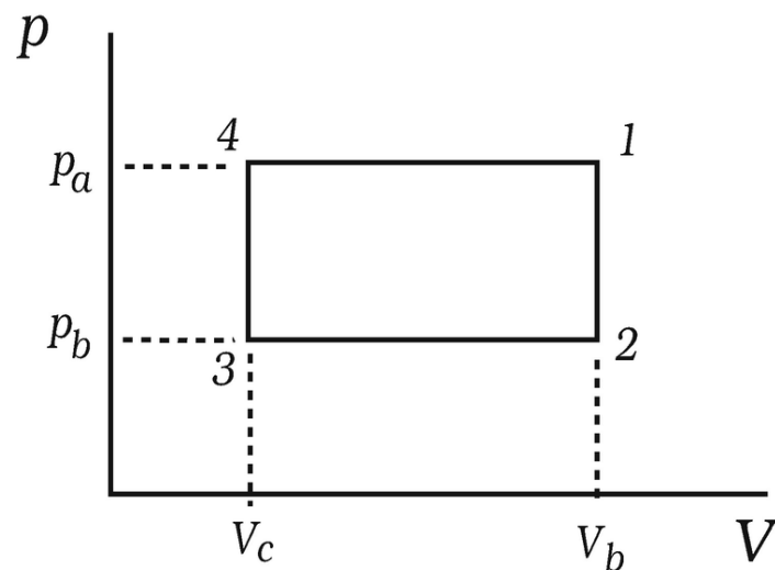
Fig. 6.2 The idealized cylinder pressure in a Newcomen engine as a function of the cylinder volume
