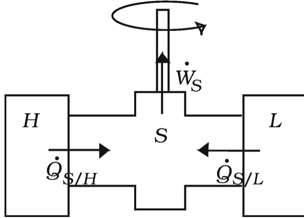
Fig. 5.4 The system considered in Theorem 5.5
