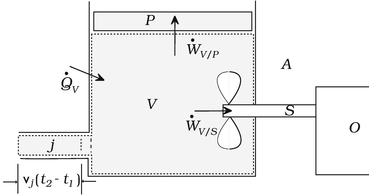
Fig. 5.2 Entropy increases in the volume V as a result of convection through the feedpipe j , and transfer from the surroundings. The surroundings, \tilde{S} consists of the air A , the piston P , and the shaft S
