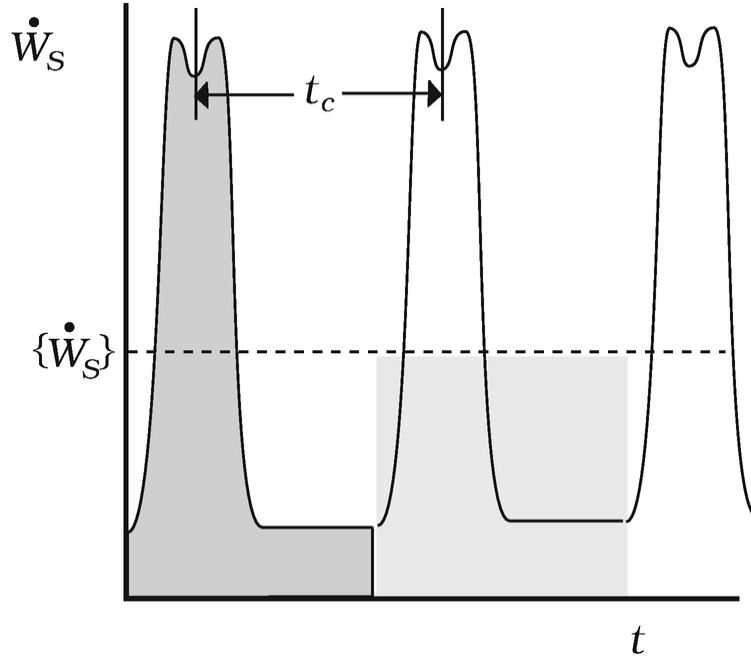
Fig. 3.5 The area under the instantaneous power curve over a cycle, W_S (dark shading), is equal to \{\dot{W}_S\}t_c (light shading) as given by Eq. (3.3)
