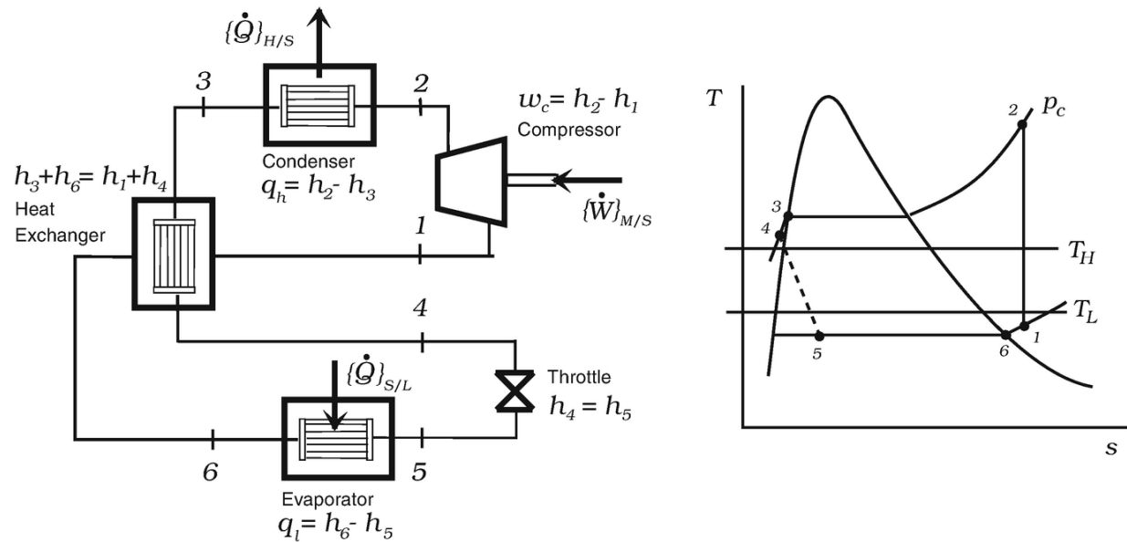
Fig. 6.22 A heat exchanger that uses subcooling the liquid to superheat the vapor in a vapor compression refrigeration cycle
