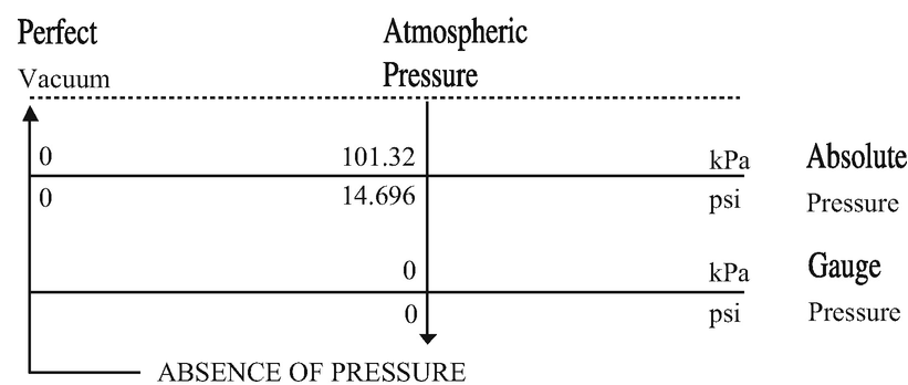
Fig. 1.6 Illustrating the relative nature of gauge pressure. Compare this with Figs. 1.2 and 1.3 that show relative distance and time
