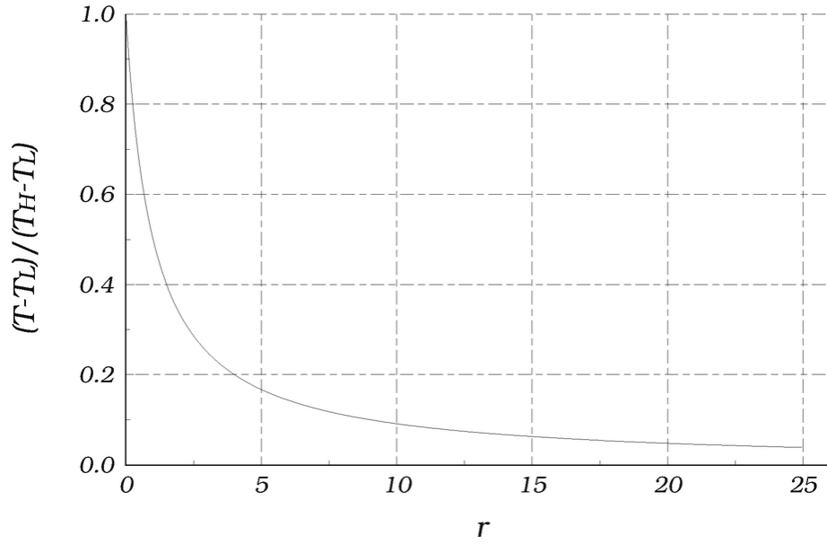
Fig. 3.10 Dimensionless representation of Eq. (3.63)
