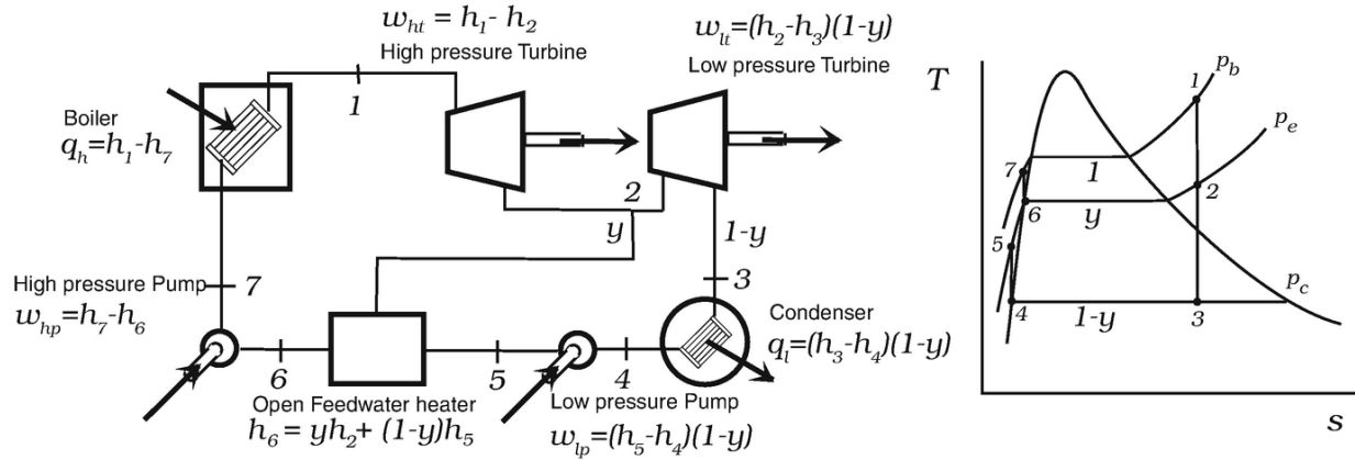
Fig. 6.8 A Rankine cycle with regeneration using an open feedwater heater is shown on the left. The state points on the T, s diagram on the right correspond to the locations shown on the left. The extraction fraction, denoted by y , is determined by requiring state 6 to be saturated liquid
