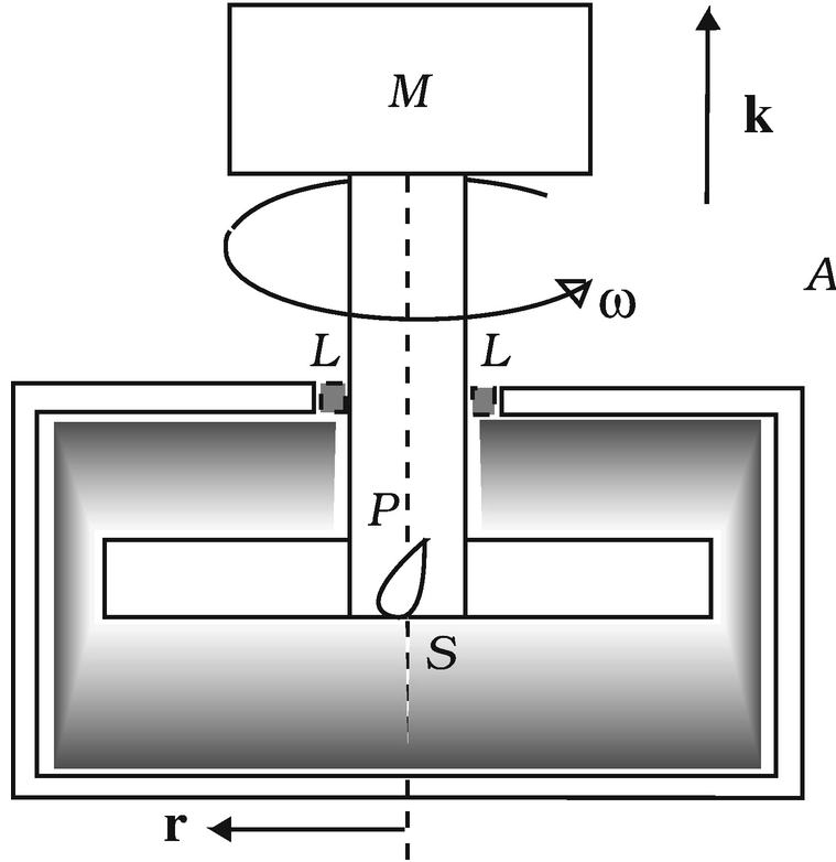
Fig. 3.6 A stirring process is an example of rigid rotational motion. The systems shown here are the stirred fluid S , the propeller P , the air A , the lubricant L , and the motor M
