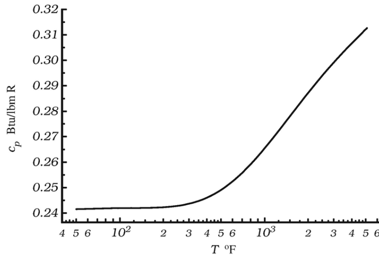
c_p Variation with Temperature
