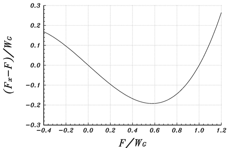
Calibration Curve Force Gauge with Cubic Spring
