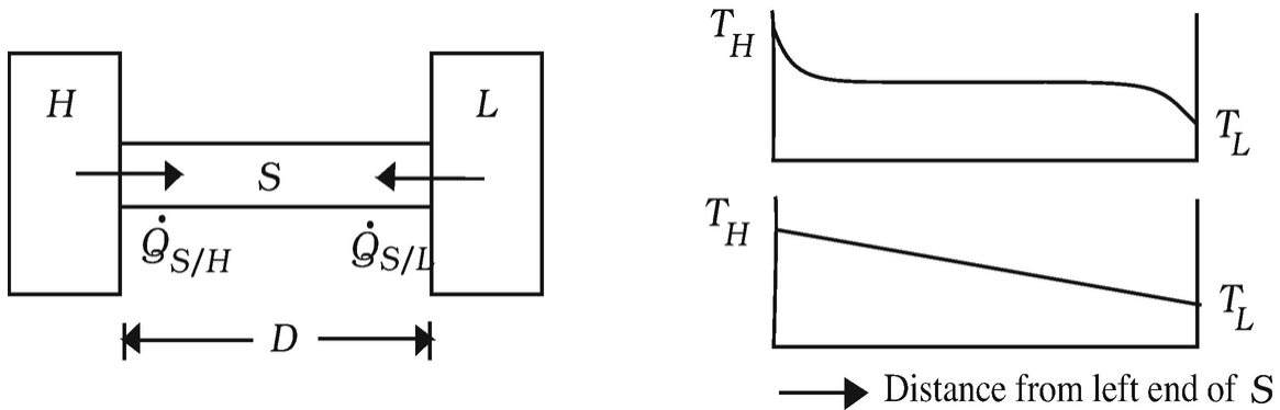
Fig. 3.9 An illustration of the heat transfer problem discussed in the text. The upper temperature distribution represents convection and occurs when S is a circulating fluid, while the lower represents conduction and occurs when S is a solid
