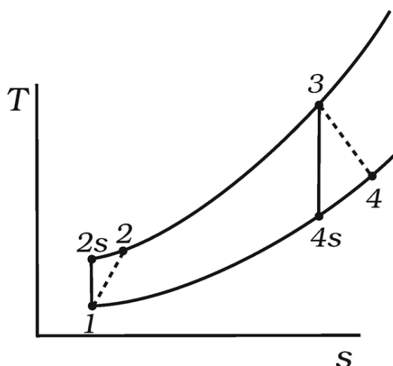
Fig. 6.18 The T - s diagram of a gas turbine power plant showing the compressor and turbine losses
