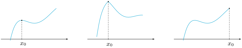
Figure 6.3. Types of maxima
