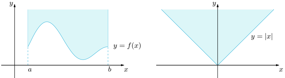
Figure 6.12. The set E_f for a generic f defined on I (left) and for f(x) = |x| (right)
