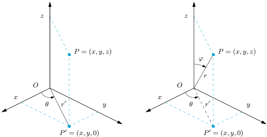
Figure 8.2. Cylindrical coordinates (left) and spherical coordinates (right)
