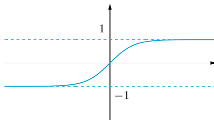
Figure 6.15. Hyperbolic tangent
