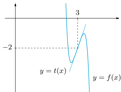
Figure 7.10. Local behaviour of the map (7.25)
