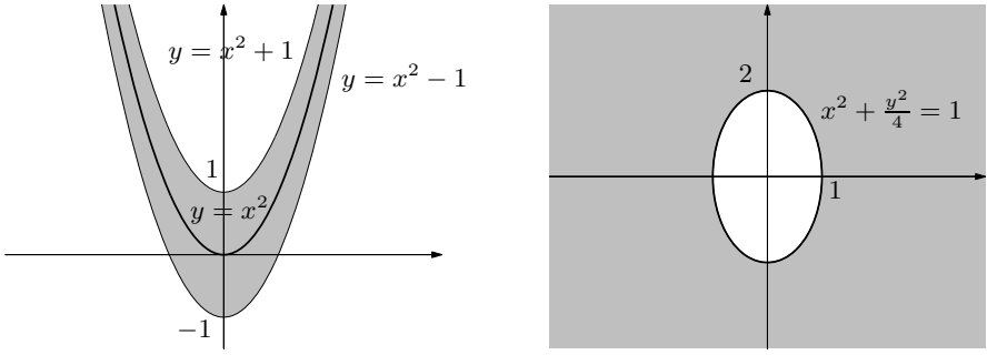
Figure 1.14. The sets C and D of Exercise 3
