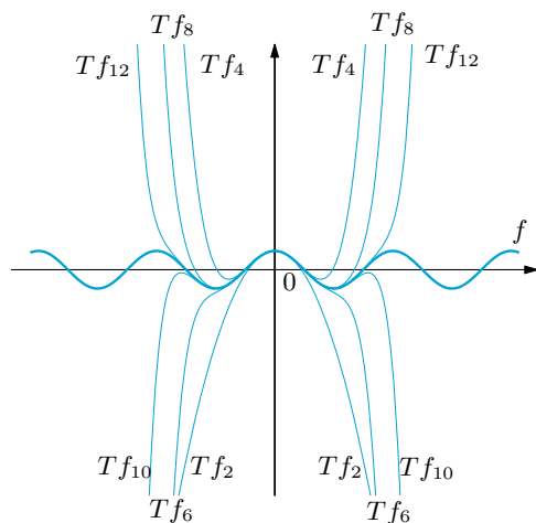
Figure 7.7. Local approximation of f(x) = \cos x by T f_{2m} = T f_{2m,0} when 1 \leq m \leq 6
