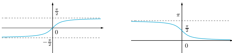
Figure 2.25. Graphs of y = \arctan x (left) and y = \operatorname{arccot} x (right)
