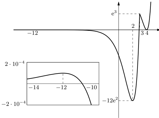
Figure 6.23. Graph of f(x) = e^x(x^2 - 8|x - 3| - 8)
