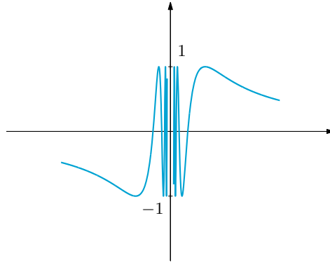
Figure 3.8. Graph of f(x) = \sin \frac{1}{x}
