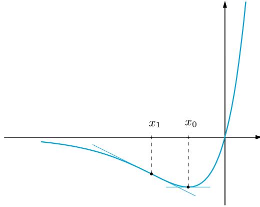
Figure 6.11. Example 6.29
