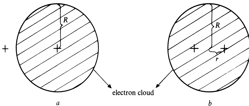
Figure 2 Two electron distributions assumed for \text{H}_2^+ .
