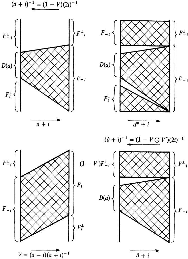
Figure 4 In the top two figures, the decomposition on the left is not assumed orthogonal. Although D(a) \cap F_{\pm i}^\perp = \{0\} , D(a) \not\subset F_{\pm i} . The extension \hat{a} , a \subset \hat{a} \subset a^* and V' are defined in (2.5.11).
