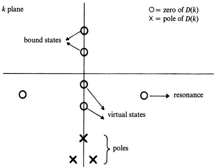
Figure 13 The configuration of the poles and zeroes of D(k) .
