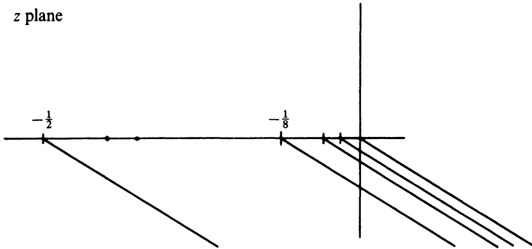
Figure 20 \text{Sp}(\exp(2\tau)\frac{1}{2}(|\mathbf{p}_1|^2 + |\mathbf{p}_2|^2) - \exp(\tau)/r_1) when \text{Im } \exp(2\tau) < 0 .
