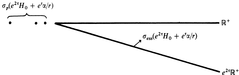
Figure 16 Spectrum of the dilated Hamiltonian.
