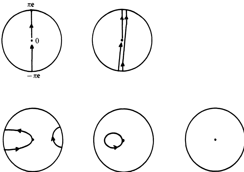
Figure 7 Homotopy of paths in \text{SO}(3) .
