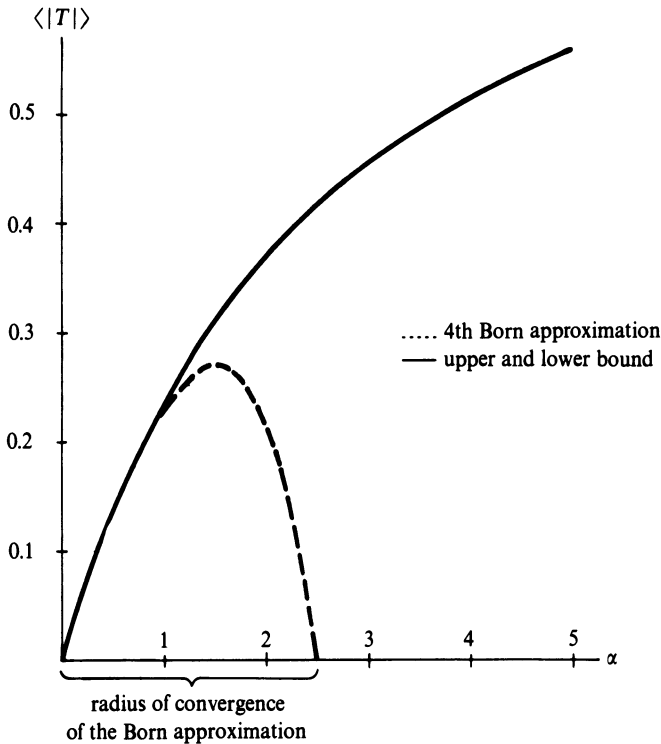
Figure 15 Bounds and approximation for the scattering length of a spherical square-well potential.
