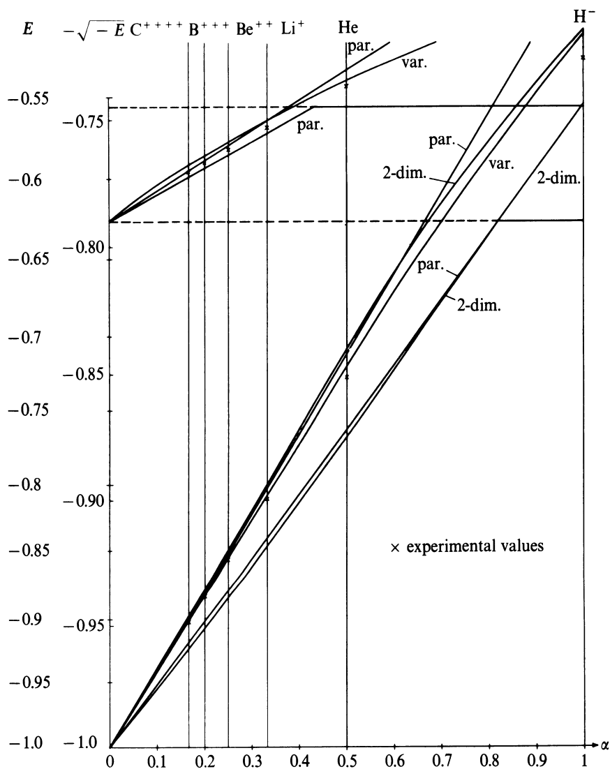
Figure 19a Variational calculation, parabolic bounds, and two-dimensional bounds for (1s)^2\ ^1S and (1s)(2s)\ ^3S .
