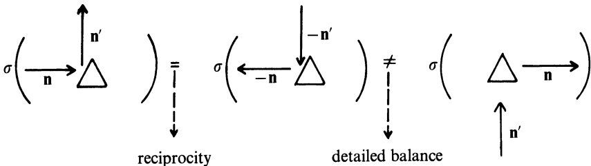
Figure 14 Scattering from a triangle.
