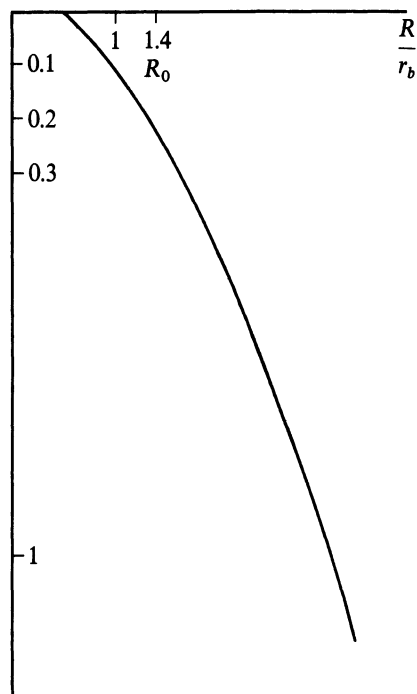
Figure 22 E \cdot R^2 in atomic units for H_2 .
