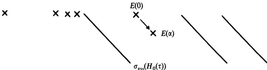
Figure 21 The motion of the eigenvalues of H_\alpha(\tau) for \alpha > 0 .
