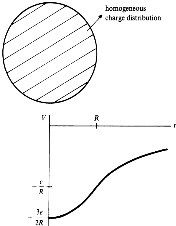
Figure 1 The potential of a homogeneous charge distribution.
