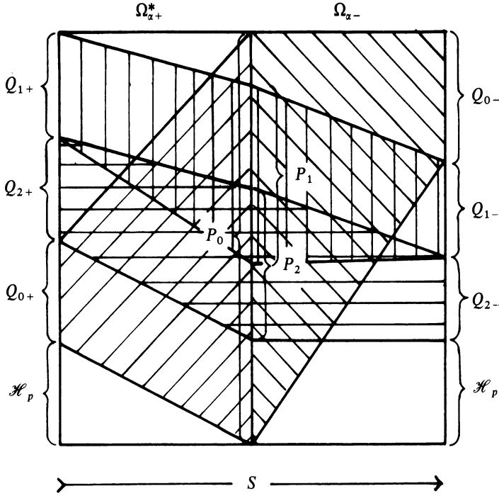
Figure 9 The domains and ranges of \Omega_{\alpha+}^* and \Omega_{\alpha-} in a system with several channels.
