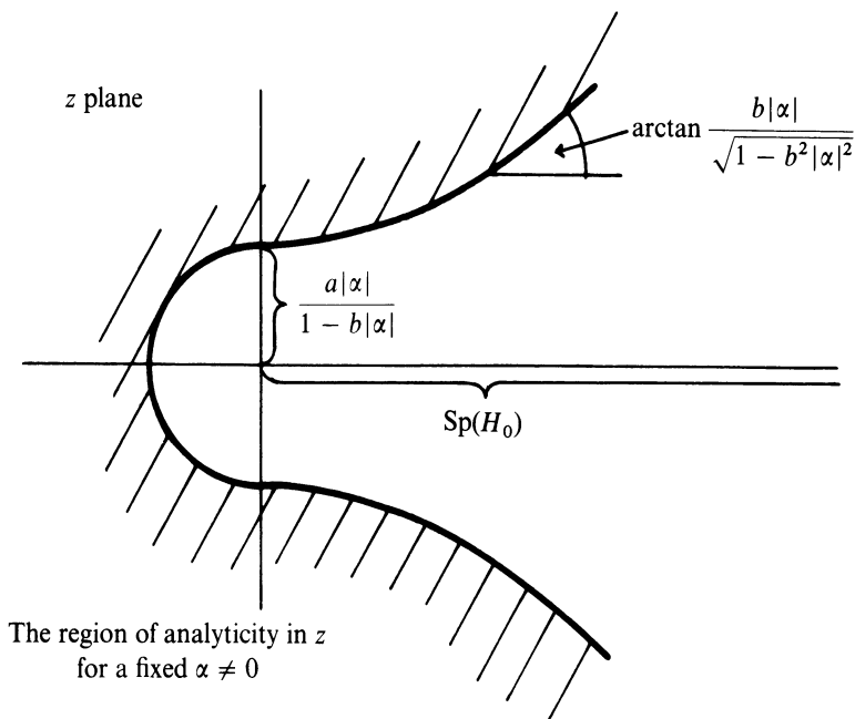
Figure 10 The region of analyticity of the resolvent.
