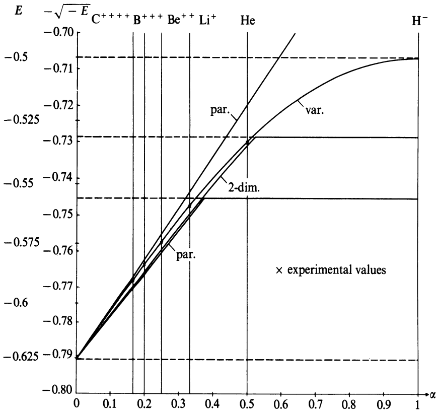
Figure 19b Variational calculation, parabolic bounds, and two-dimensional bounds for (1s)(2p) \ ^3P .
