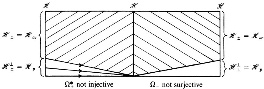
Figure 8 The domains and ranges of \Omega^* and \Omega .
