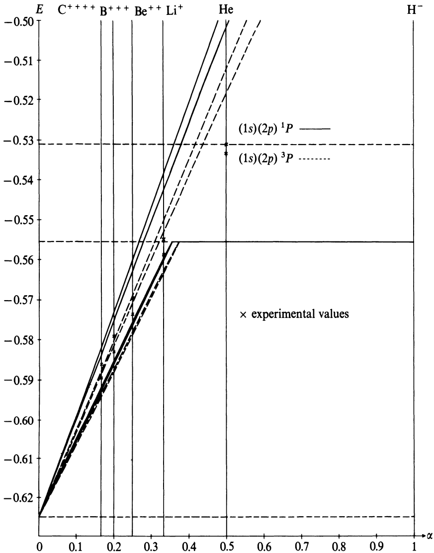
Figure 18 Linear and parabolic bounds for (1s)(2p) \ ^3P and (1s)(2p) \ ^1P .
