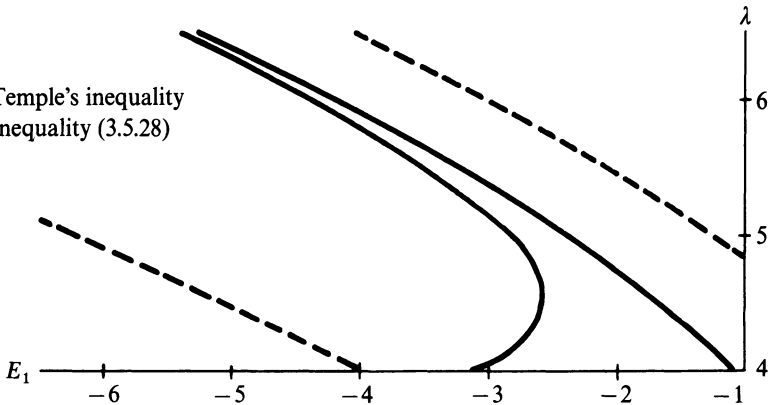
Figure 12 Bounds for the ground state with a Yukawa potential.
