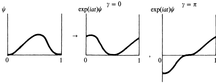
Figure 5 Two unitary representations of the translation on [0, 1] .
