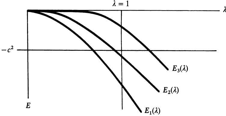
Figure 11 The eigenvalues as functions of the coupling constant.
