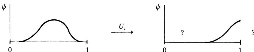
Figure 3 Unitary representation of the translation on [0, 1] .
