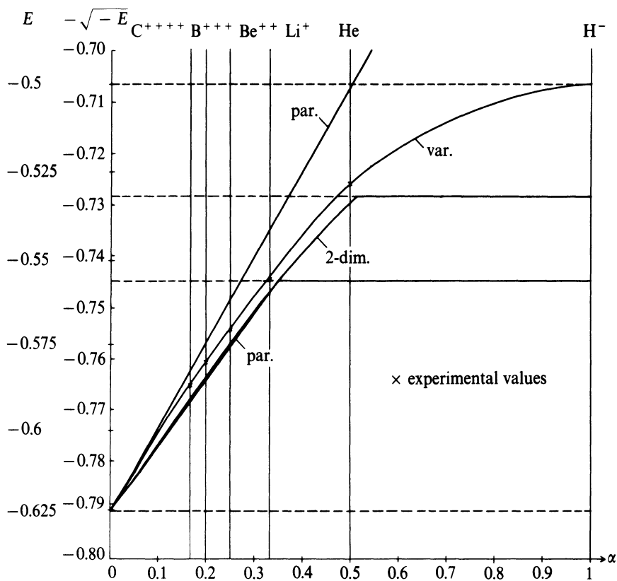
Figure 19c Variational calculation, parabolic bounds, and two-dimensional bounds for (1s)(2p) {}^1P .
