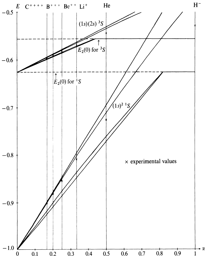
Figure 17 Linear and parabolic bounds for (1s)^2 \ ^1S and (1s)(2s) \ ^3S .
