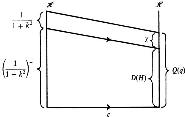
Figure 6 The domains involved in the extension of a quadratic form.
