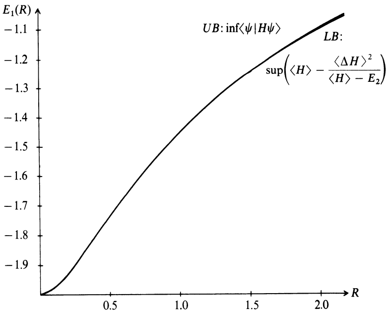
Figure 23 Bounds to E_1(R) for H_2^+ .
